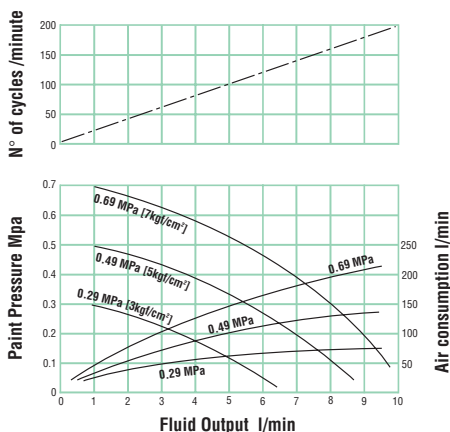
DPS 90 Performance Curve
